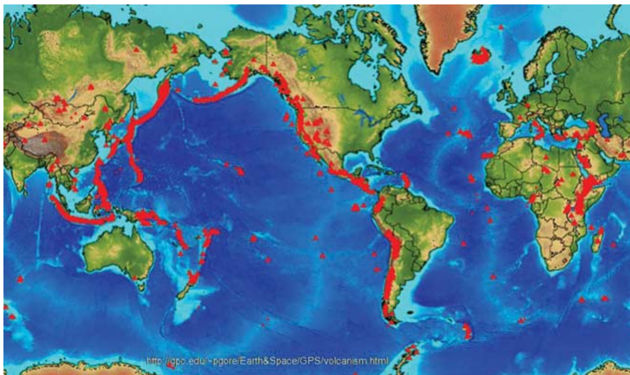
Figure 1. The 'rings of fire': distribution of active volcanoes around the world.
